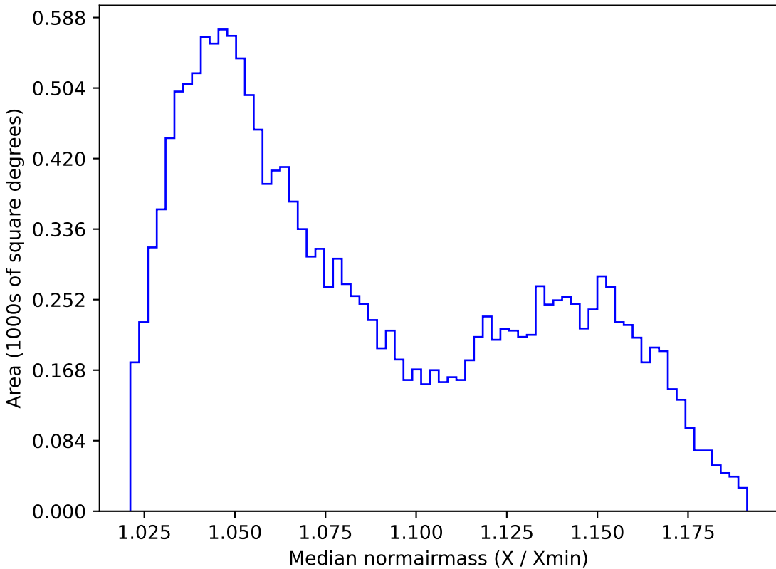
too_10_4v3.4_10yrs WFD z band: Median normairmass
