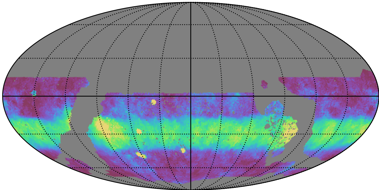
too_10_4v3.4_10yrs WFD y band: Median normairmass
