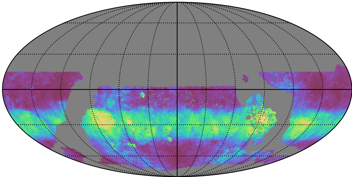
too_10_4v3.4_10yrs WFD u band: Median normairmass
