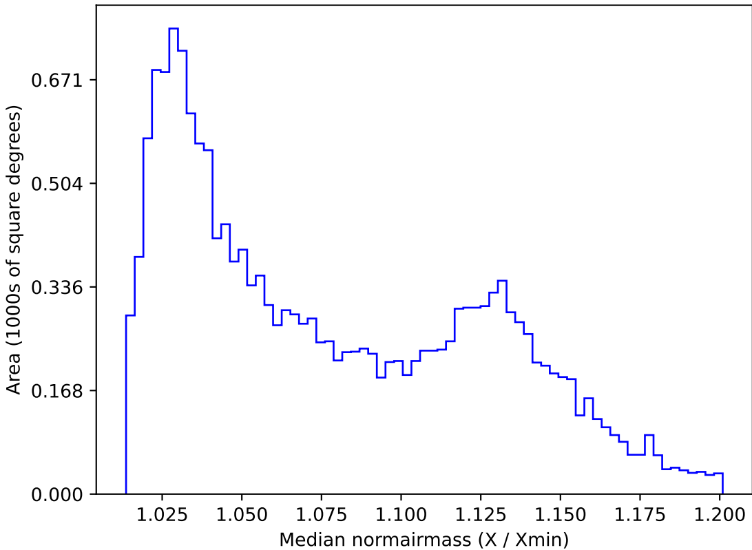
too_10_4v3.4_10yrs WFD u band: Median normairmass
