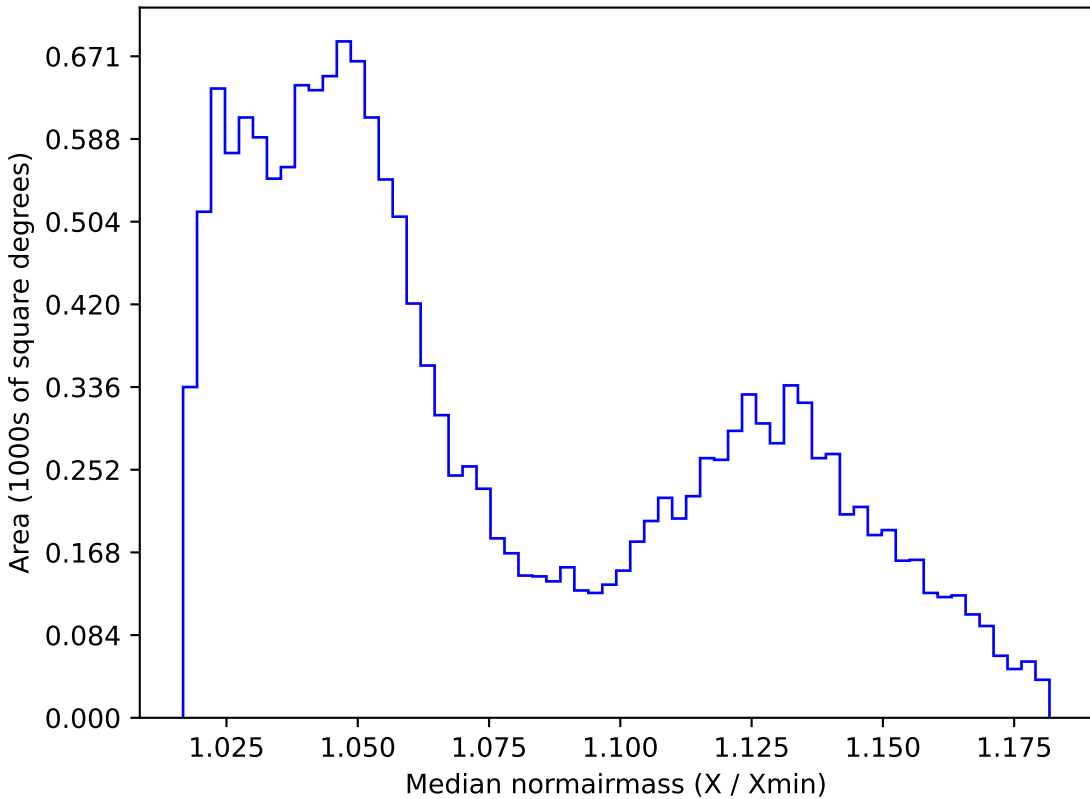
too_10_4v3.4_10yrs WFD r band: Median normairmass
