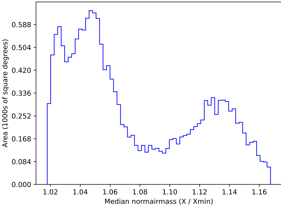
too_10_4v3.4_10yrs WFD i band: Median normairmass
