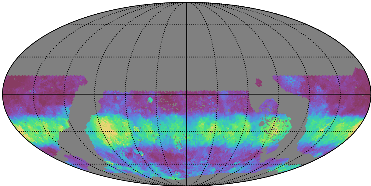
too_10_4v3.4_10yrs WFD g band: Median normairmass
