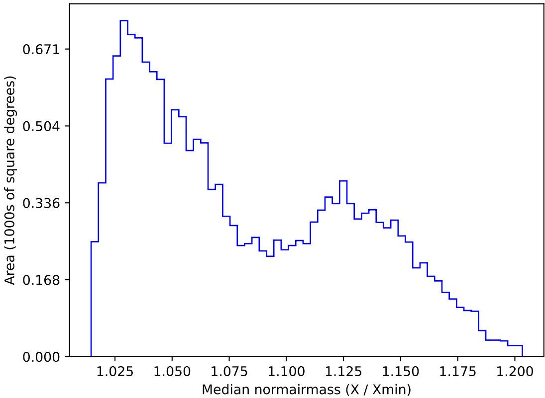
too_10_4v3.4_10yrs WFD g band: Median normairmass
