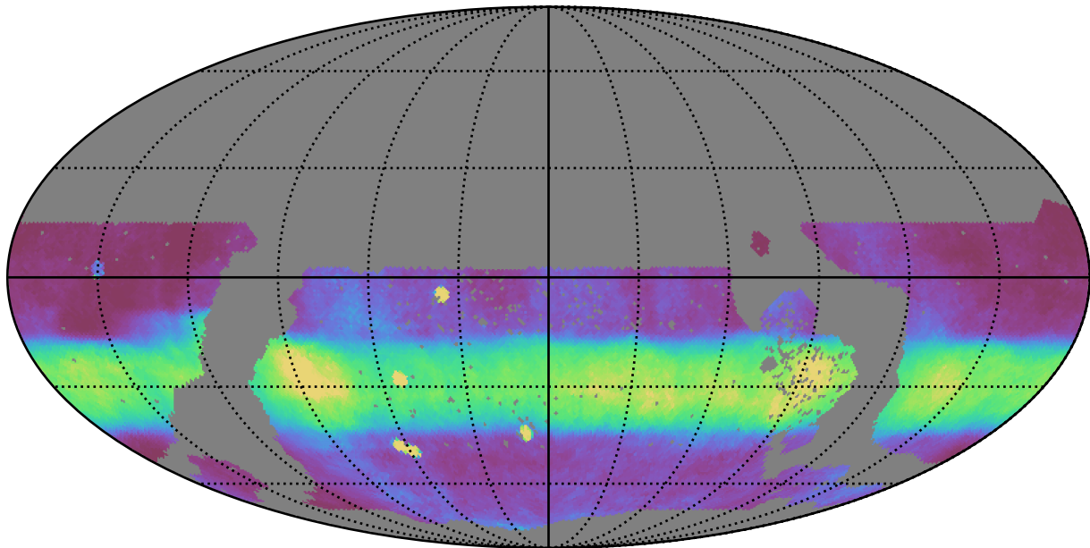
too_10_4v3.4_10yrs WFD all bands: Median normairmass
