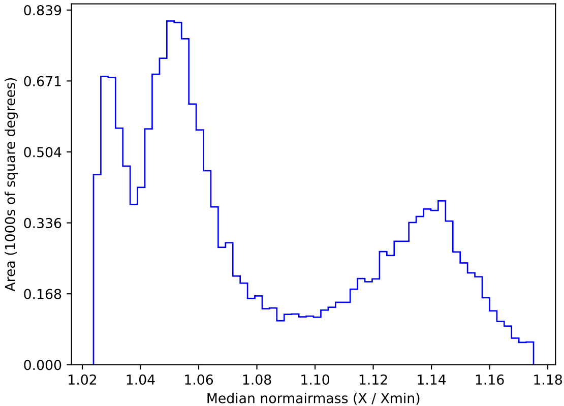
too_10_4v3.4_10yrs WFD all bands: Median normairmass
