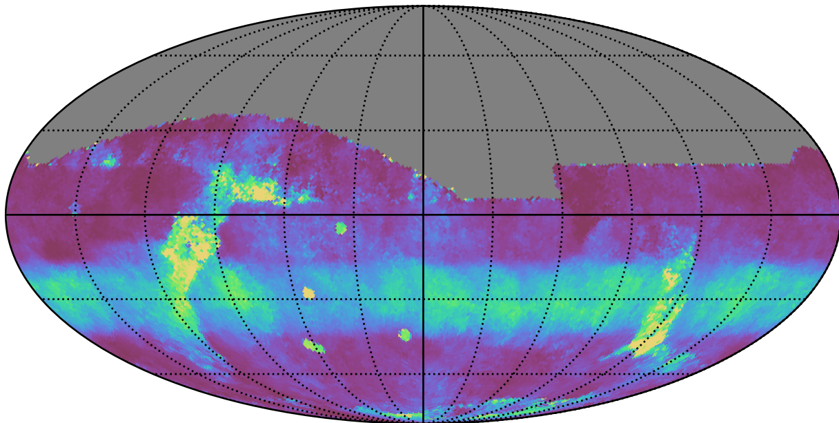
too_10_4v3.4_10yrs All sky z band: Median normairmass
