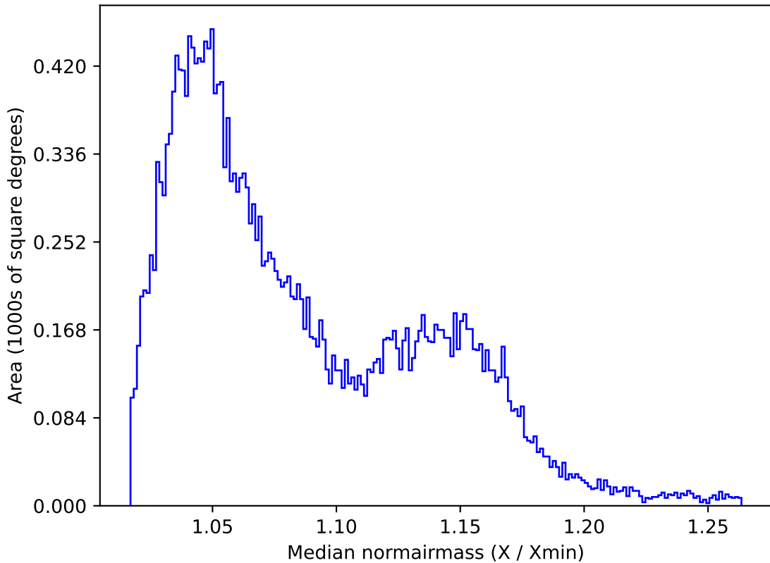
too_10_4v3.4_10yrs All sky z band: Median normairmass
