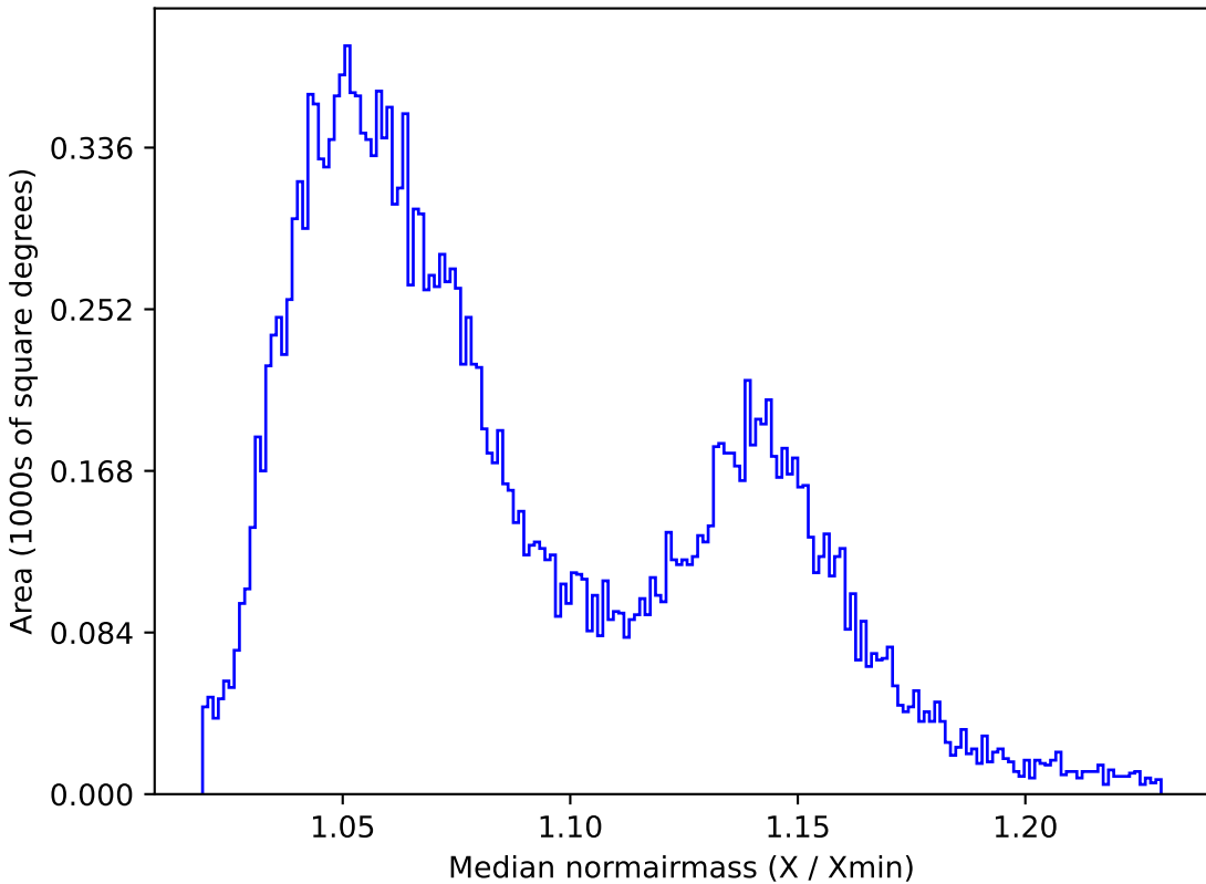
too_10_4v3.4_10yrs All sky y band: Median normairmass
