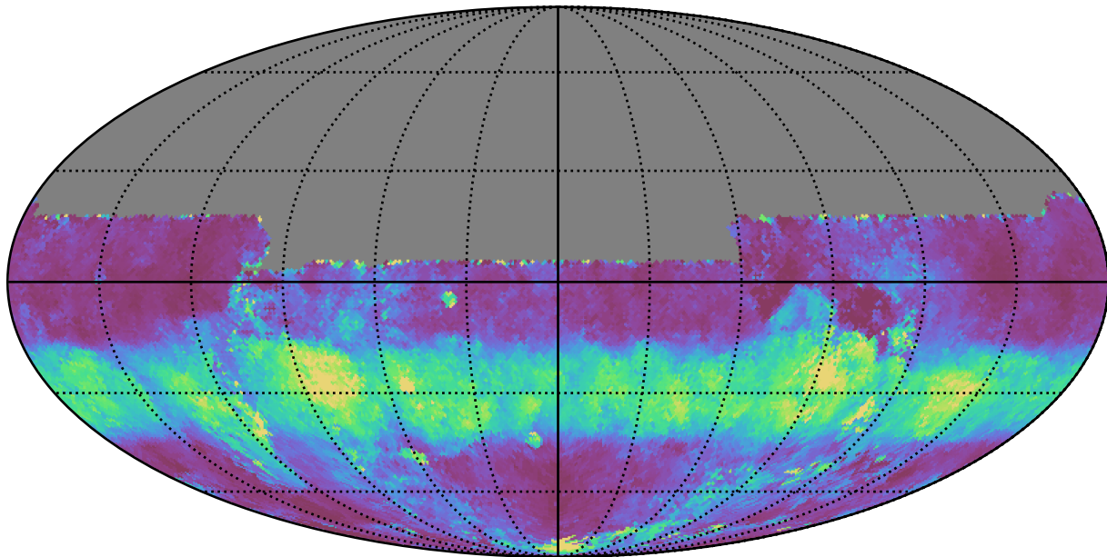
too_10_4v3.4_10yrs All sky u band: Median normairmass
