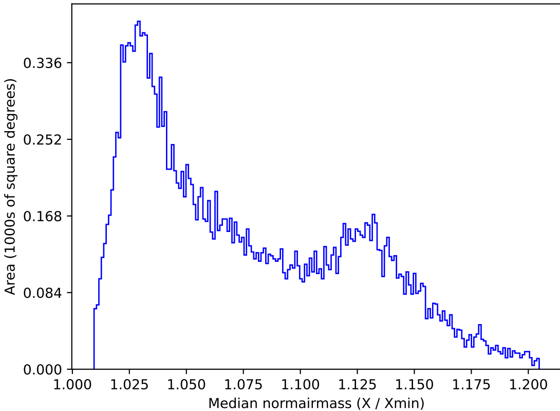
too_10_4v3.4_10yrs All sky u band: Median normairmass
