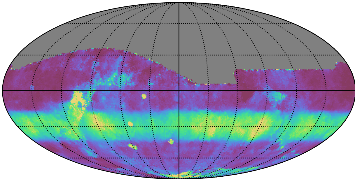
too_10_4v3.4_10yrs All sky r band: Median normairmass
