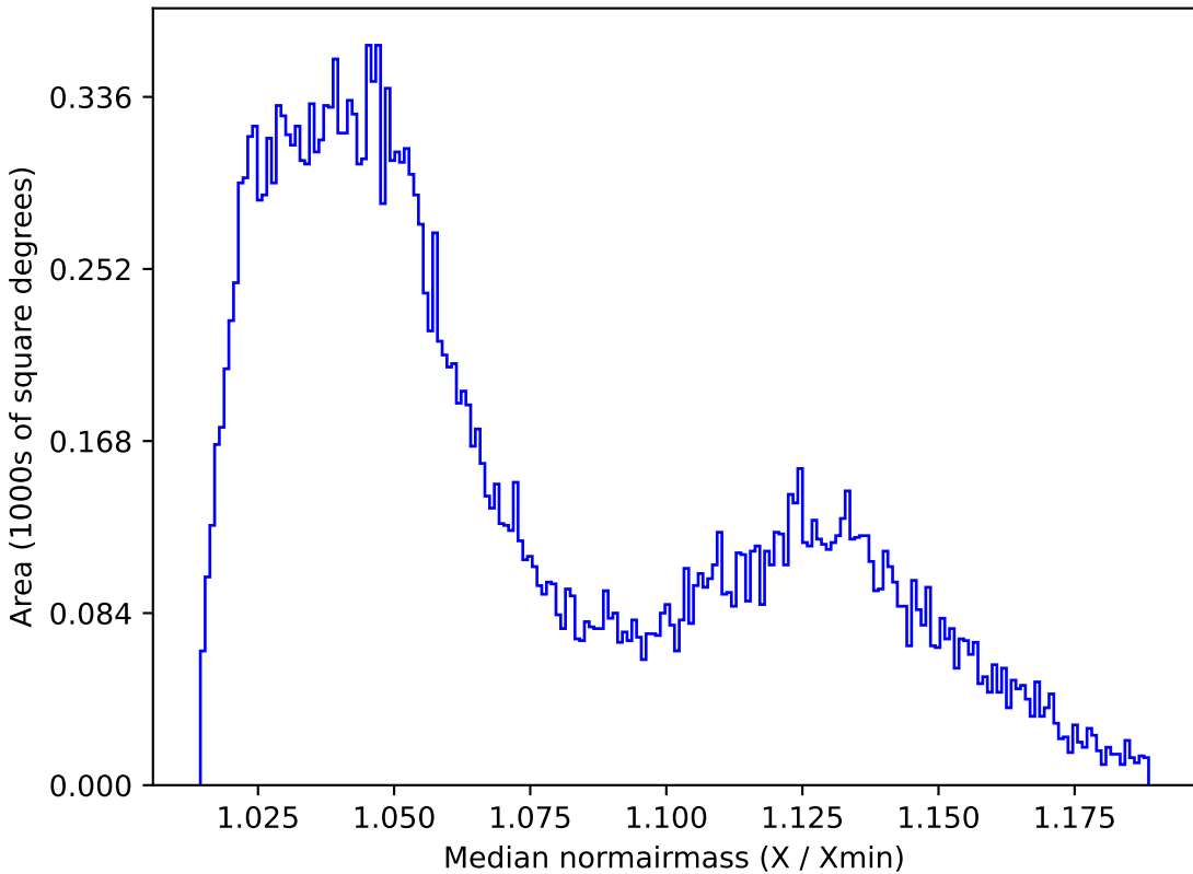
too_10_4v3.4_10yrs All sky r band: Median normairmass
