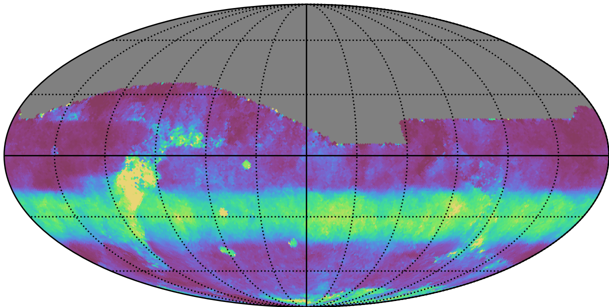
too_10_4v3.4_10yrs All sky i band: Median normairmass
