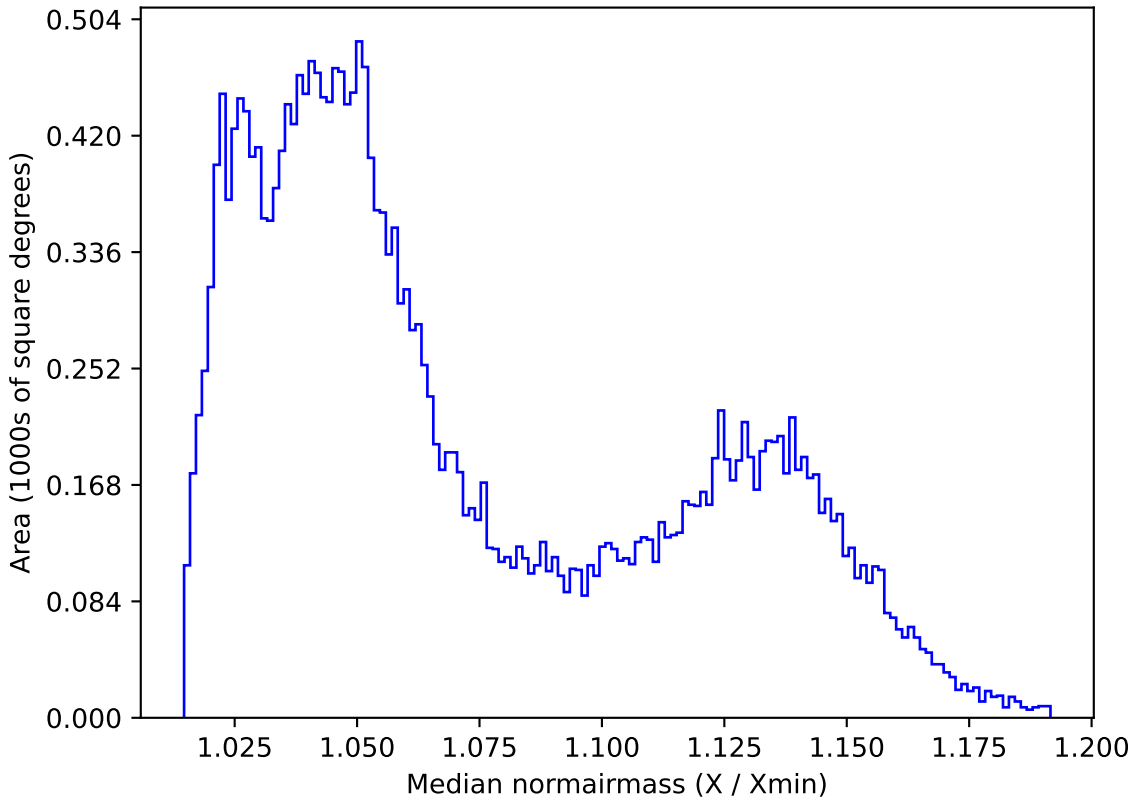
too_10_4v3.4_10yrs All sky i band: Median normairmass
