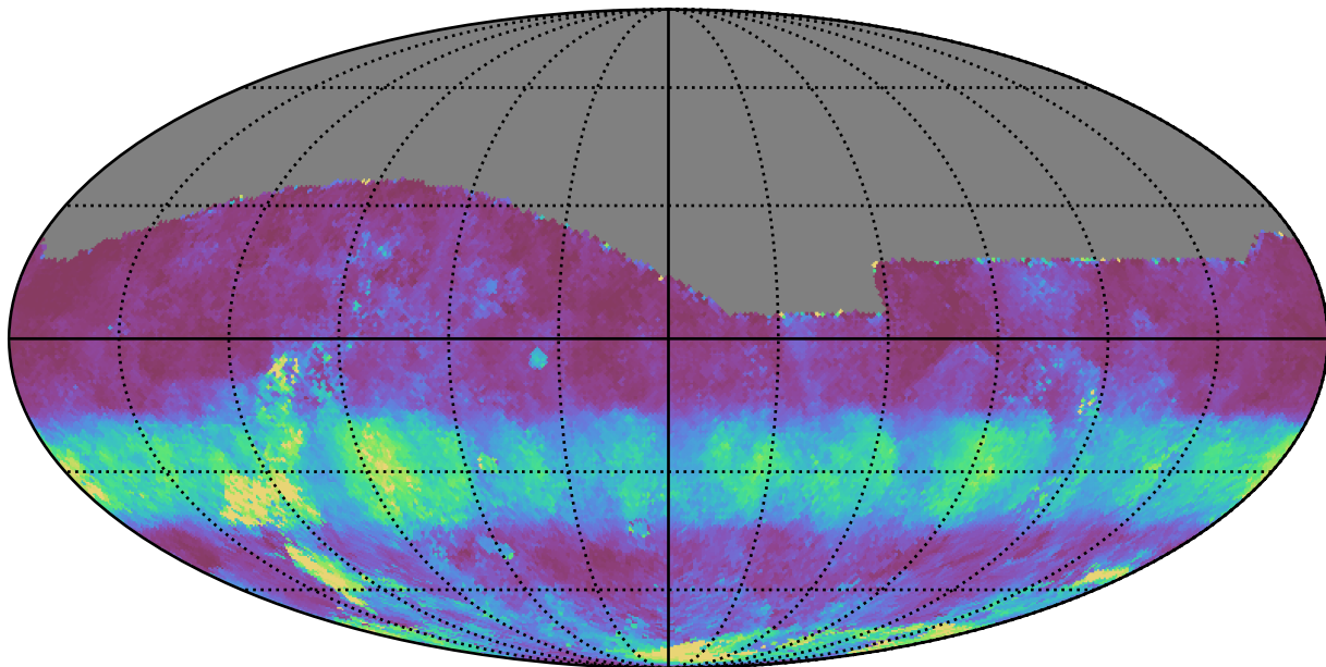
too_10_4v3.4_10yrs All sky g band: Median normairmass
