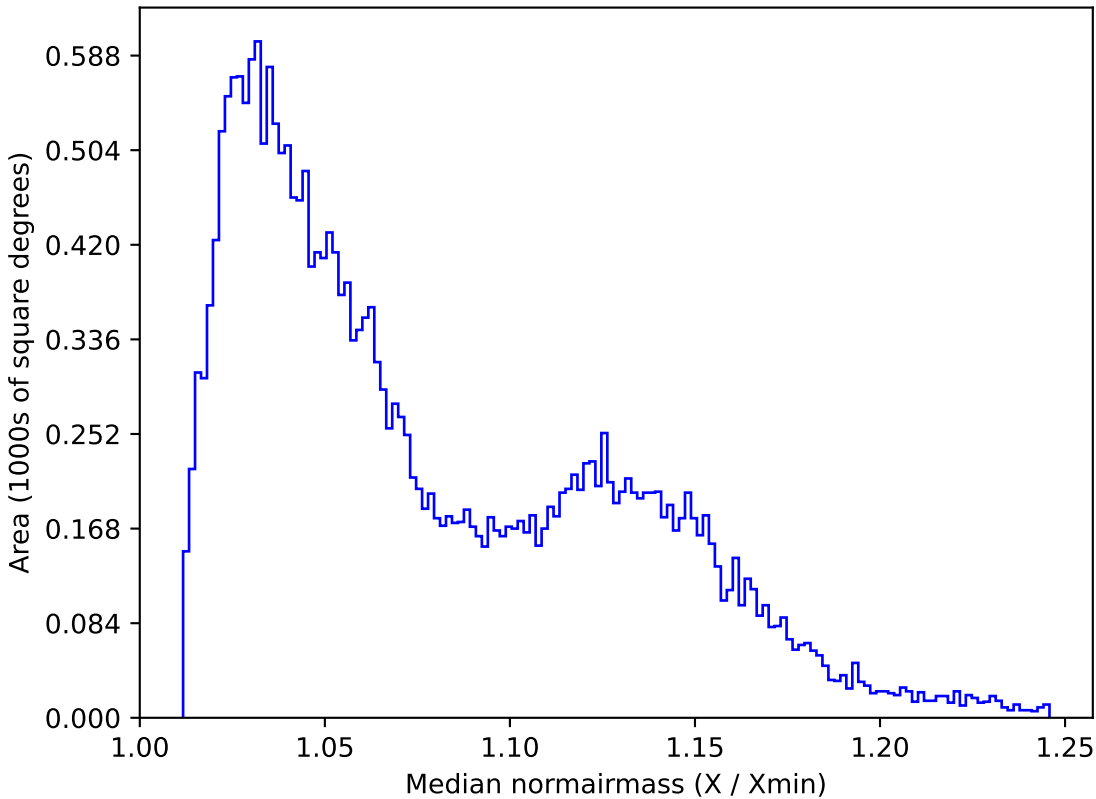
too_10_4v3.4_10yrs All sky g band: Median normairmass
