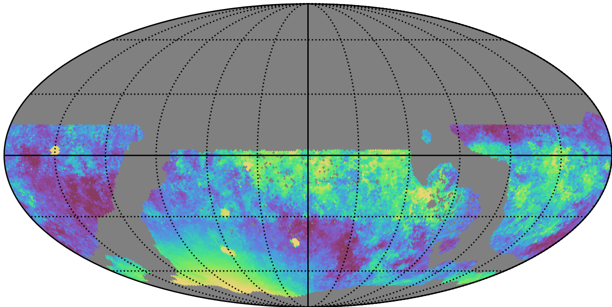
too_10_4v3.4_10yrs WFD z band: Median moonDistance
