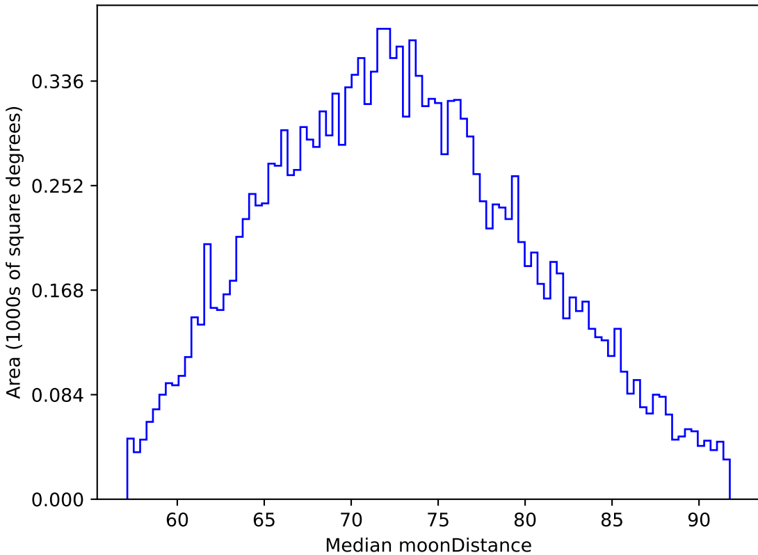
too_10_4v3.4_10yrs WFD z band: Median moonDistance
