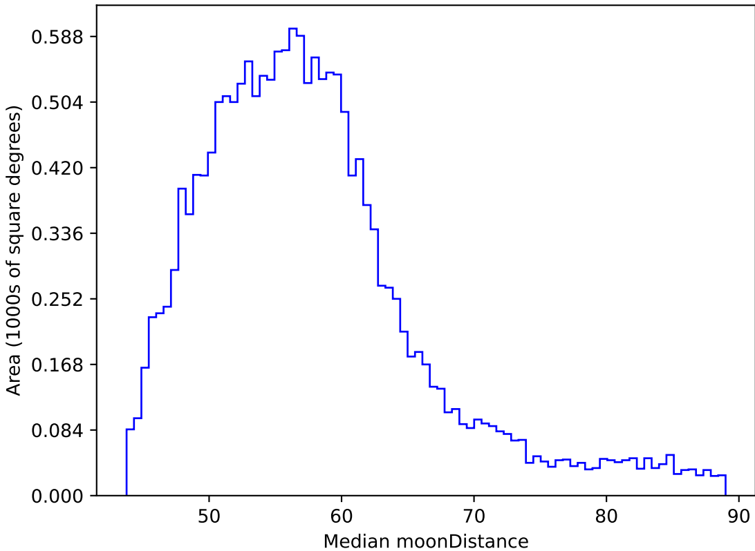
too_10_4v3.4_10yrs WFD y band: Median moonDistance
