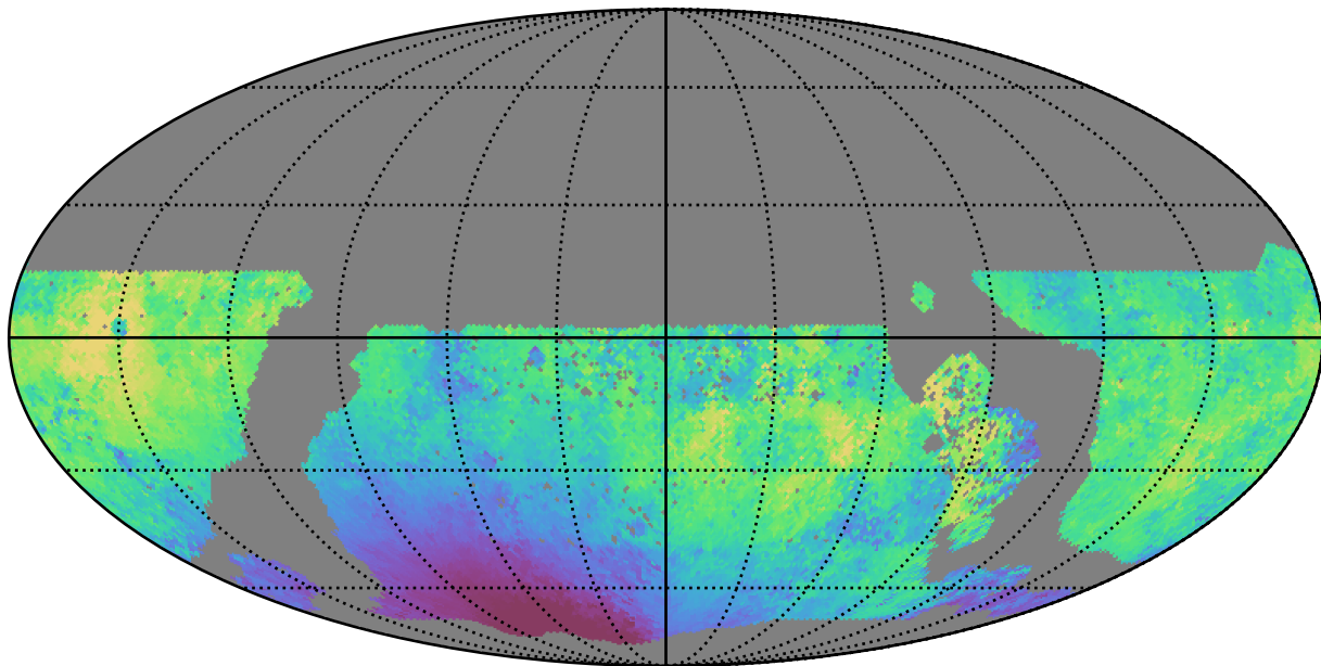
too_10_4v3.4_10yrs WFD u band: Median moonDistance
