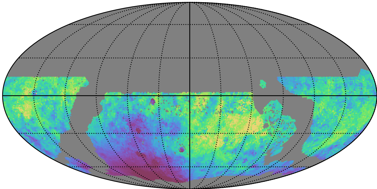
too_10_4v3.4_10yrs WFD r band: Median moonDistance
