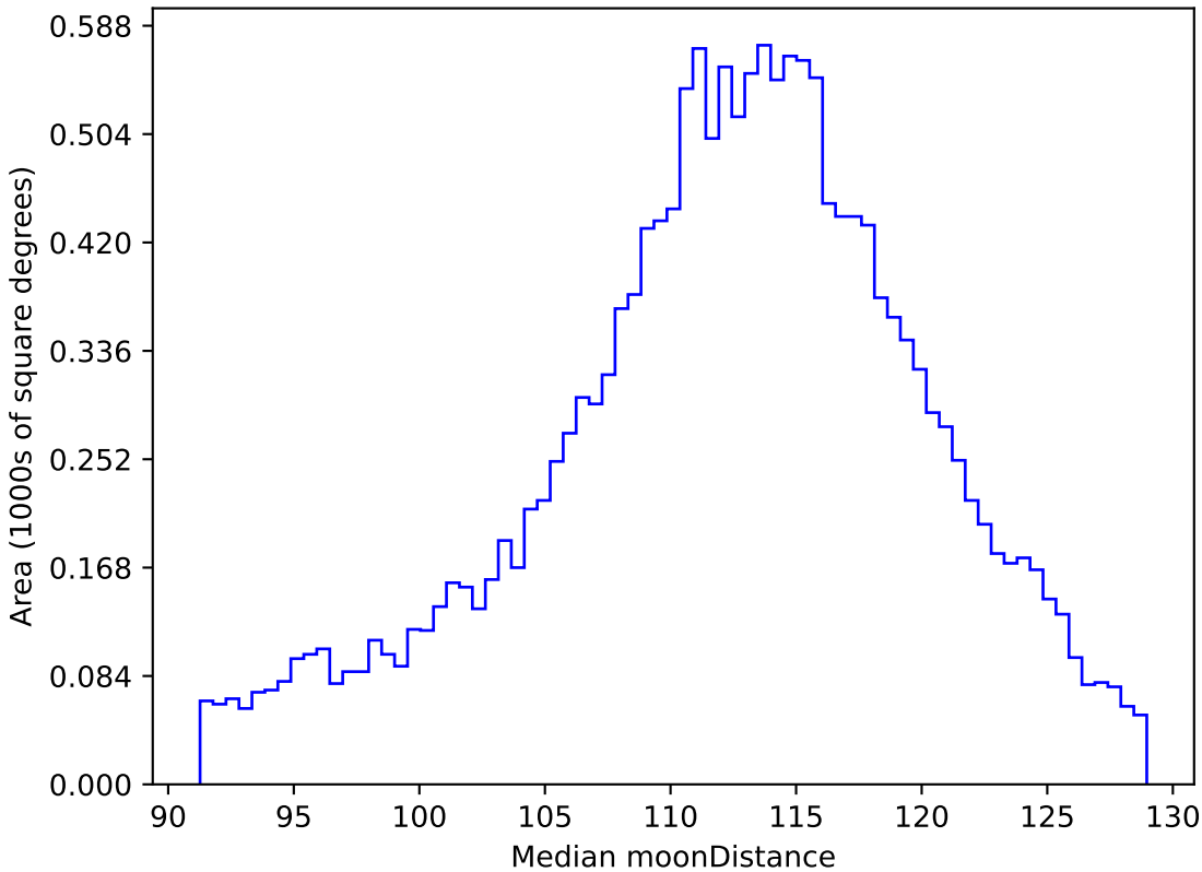
too_10_4v3.4_10yrs WFD r band: Median moonDistance
