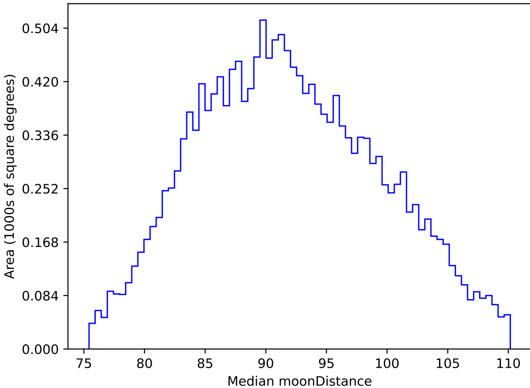
too_10_4v3.4_10yrs WFD i band: Median moonDistance
