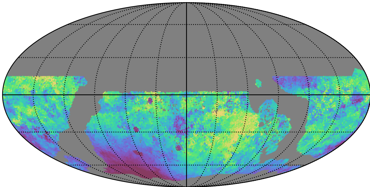
too_10_4v3.4_10yrs WFD g band: Median moonDistance
