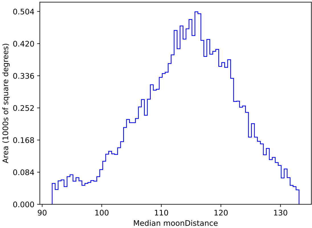
too_10_4v3.4_10yrs WFD g band: Median moonDistance
