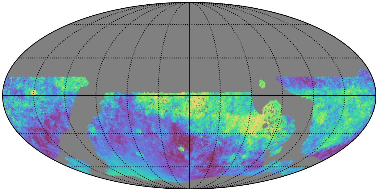
too_10_4v3.4_10yrs WFD all bands: Median moonDistance
