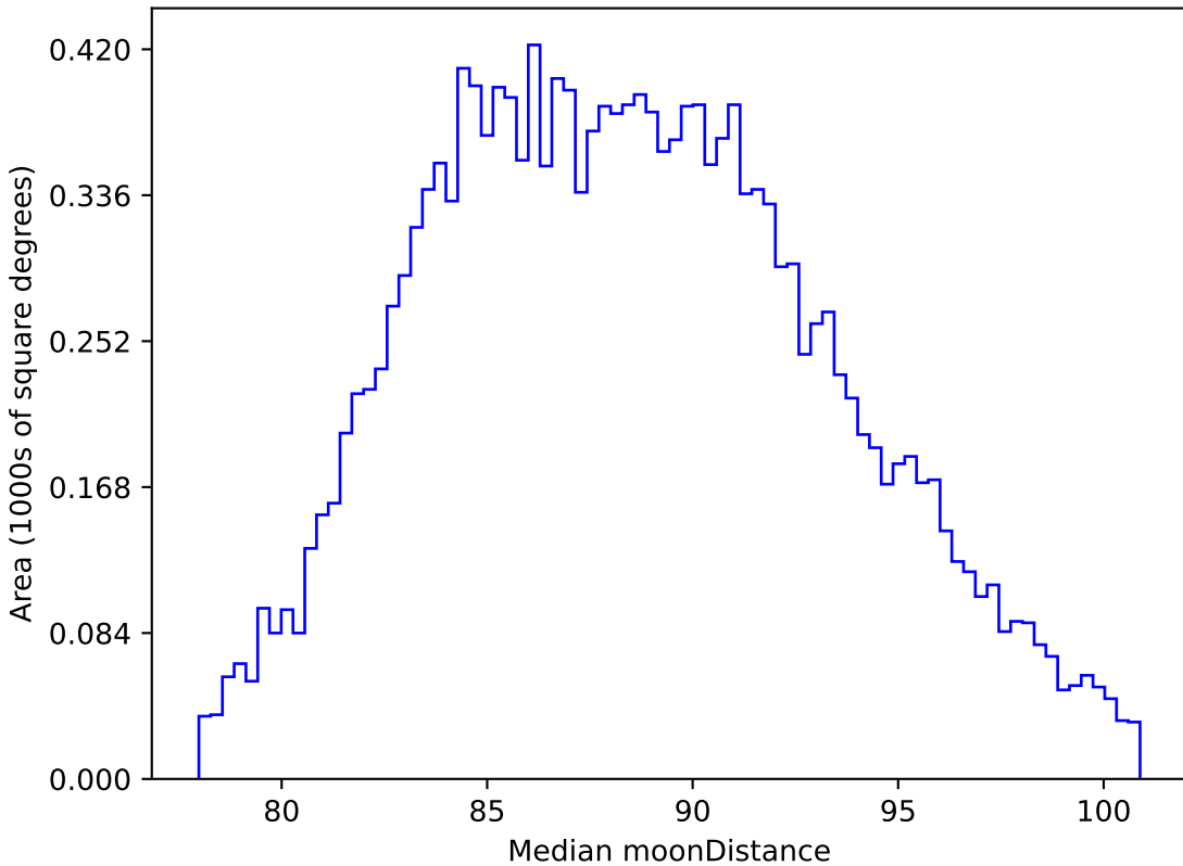
too_10_4v3.4_10yrs WFD all bands: Median moonDistance
