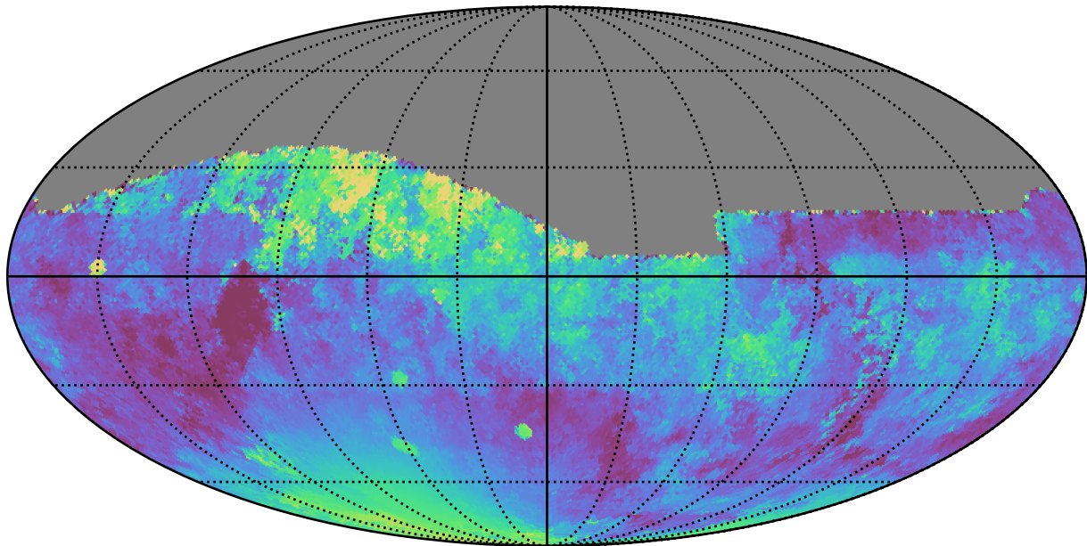
too_10_4v3.4_10yrs All sky z band: Median moonDistance
