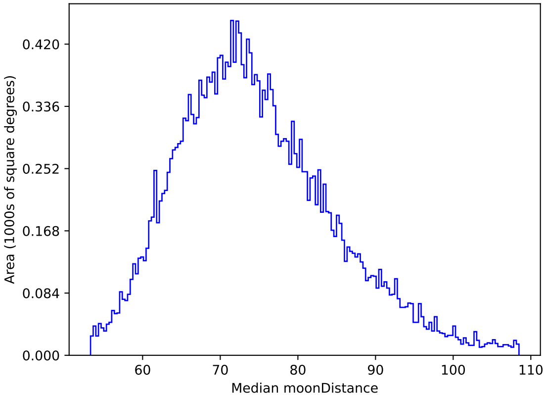
too_10_4v3.4_10yrs All sky z band: Median moonDistance
