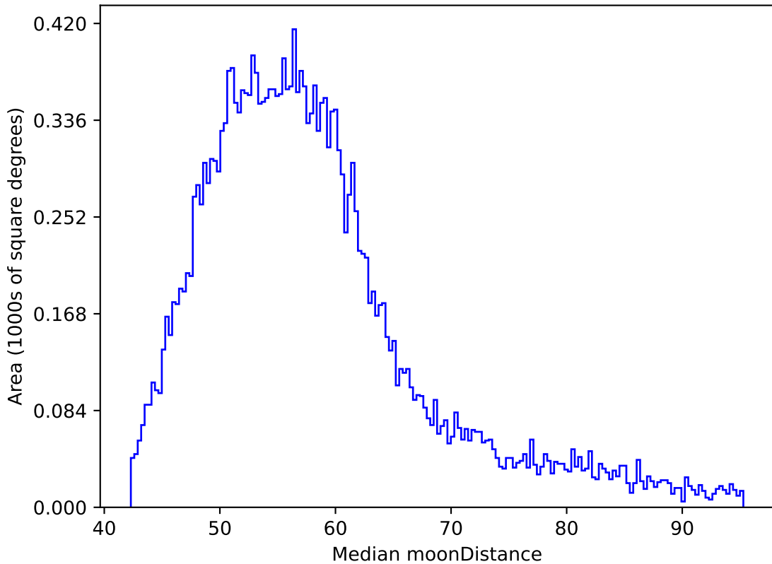
too_10_4v3.4_10yrs All sky y band: Median moonDistance
