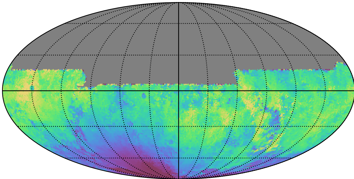
too_10_4v3.4_10yrs All sky u band: Median moonDistance
