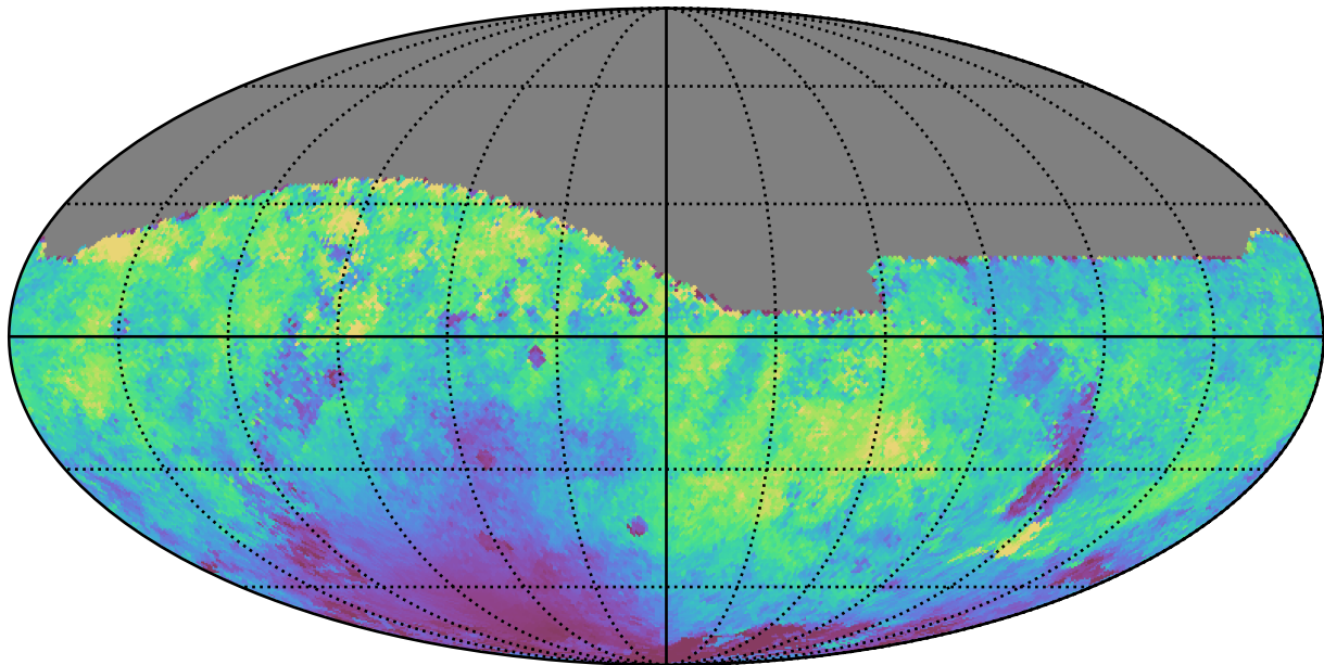
too_10_4v3.4_10yrs All sky r band: Median moonDistance
