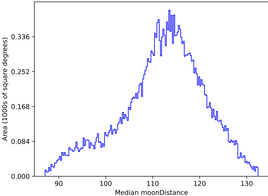
too_10_4v3.4_10yrs All sky r band: Median moonDistance
