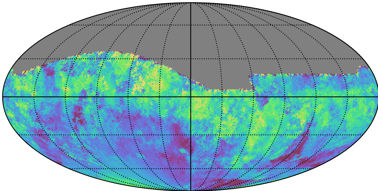
too_10_4v3.4_10yrs All sky i band: Median moonDistance
