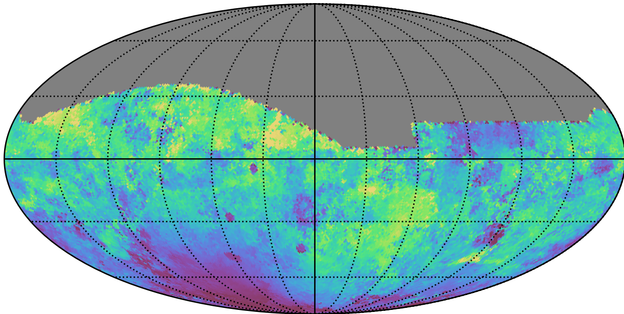
too_10_4v3.4_10yrs All sky g band: Median moonDistance
