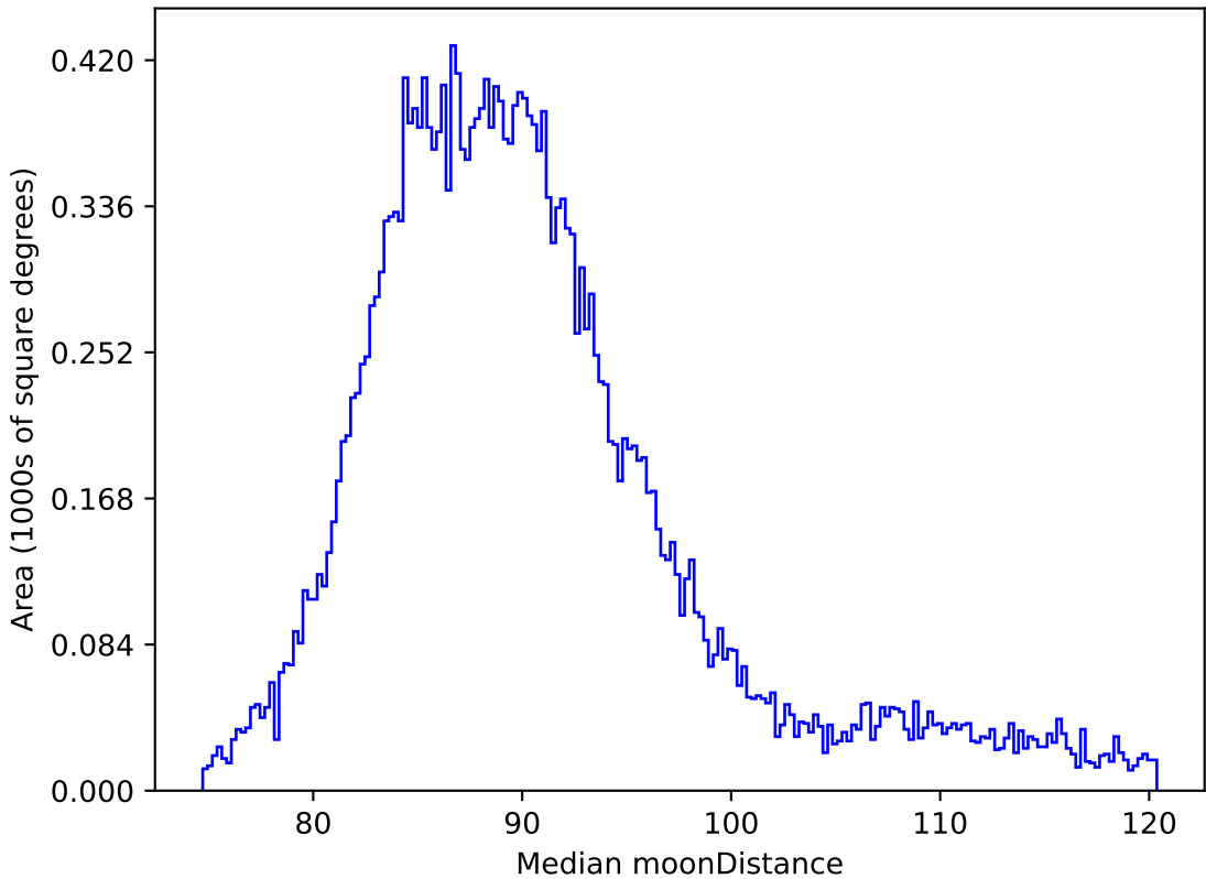
too_10_4v3.4_10yrs All sky all bands: Median moonDistance
