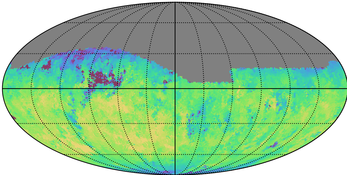
too_10_4v3.4_10yrs Yr 1 z band: Median fiveSigmaDepth
