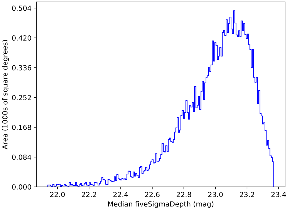
too_10_4v3.4_10yrs Yr 1 z band: Median fiveSigmaDepth
