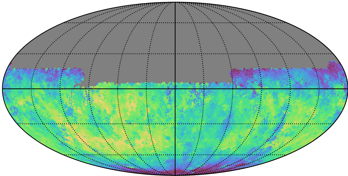
too_10_4v3.4_10yrs Yr 1 y band: Median fiveSigmaDepth
