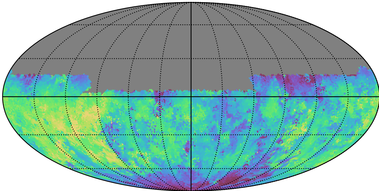
too_10_4v3.4_10yrs Yr 1 u band: Median fiveSigmaDepth
