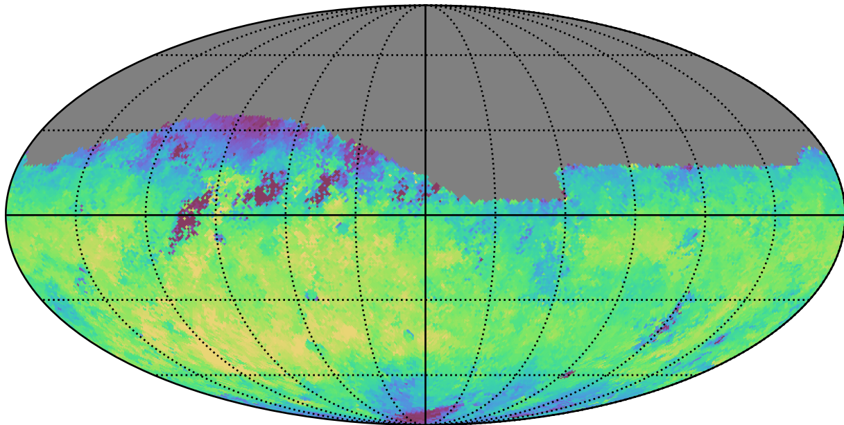
too_10_4v3.4_10yrs Yr 1 r band: Median fiveSigmaDepth
