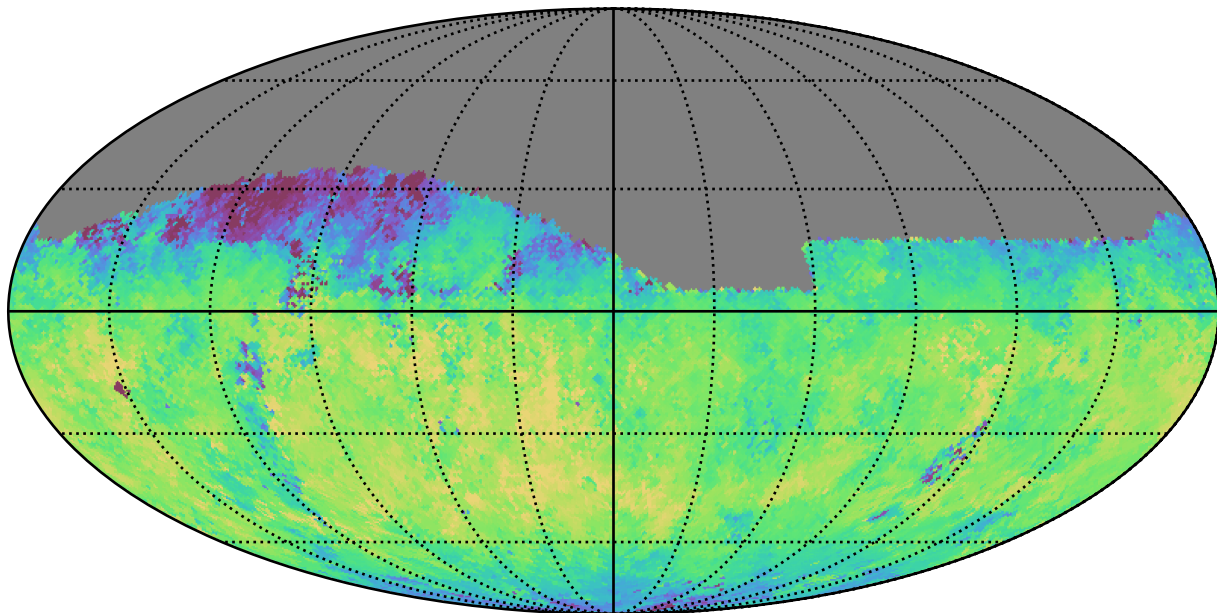
too_10_4v3.4_10yrs Yr 1 i band: Median fiveSigmaDepth
