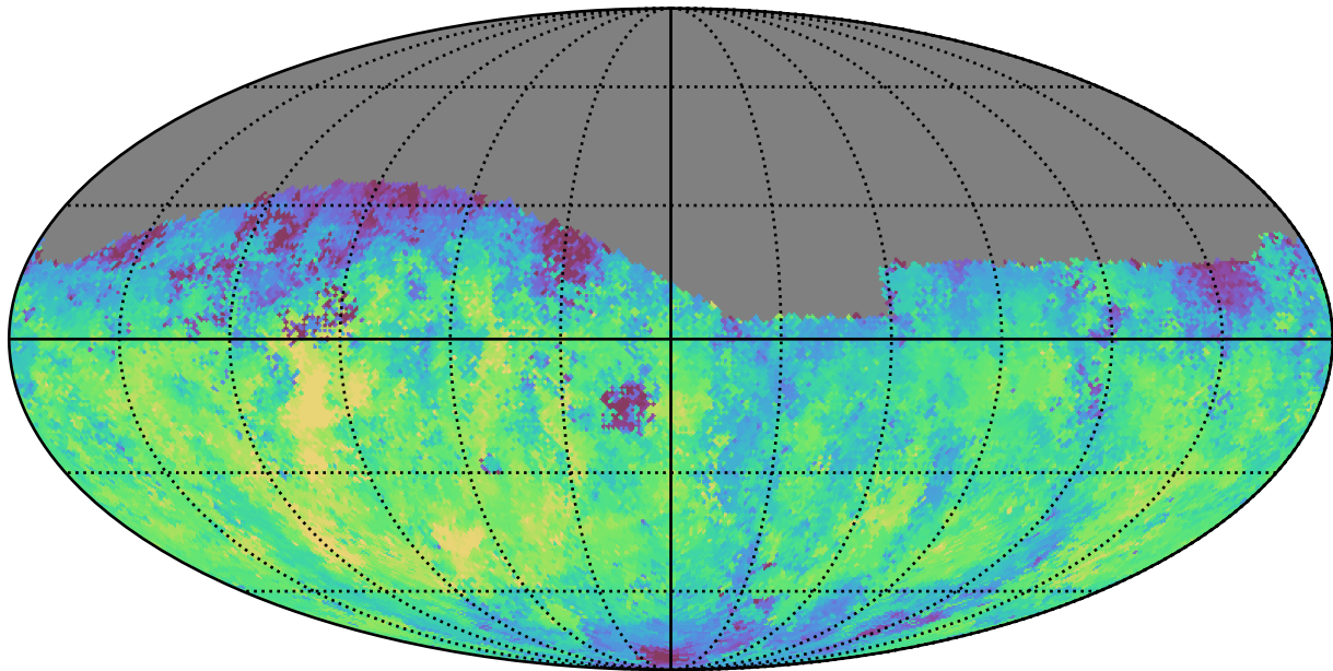
too_10_4v3.4_10yrs Yr 1 g band: Median fiveSigmaDepth
