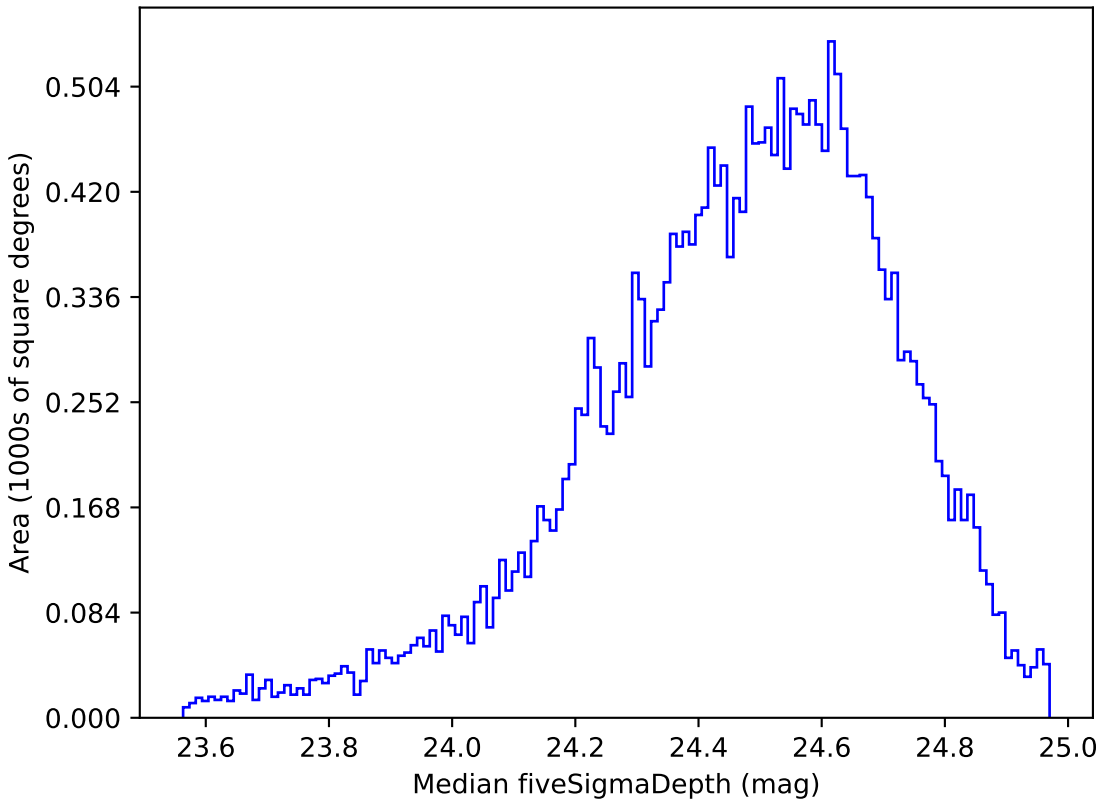
too_10_4v3.4_10yrs Yr 1 g band: Median fiveSigmaDepth
