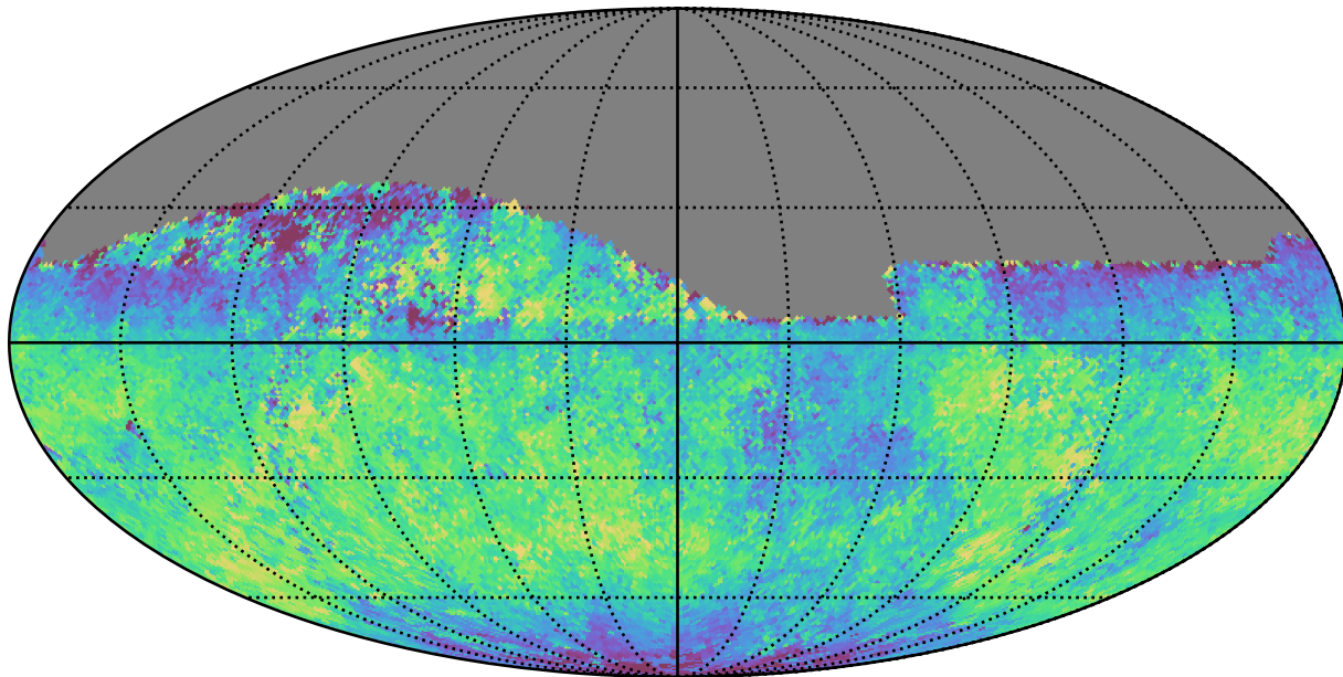
too_10_4v3.4_10yrs Yr 1 all bands: Median fiveSigmaDepth
